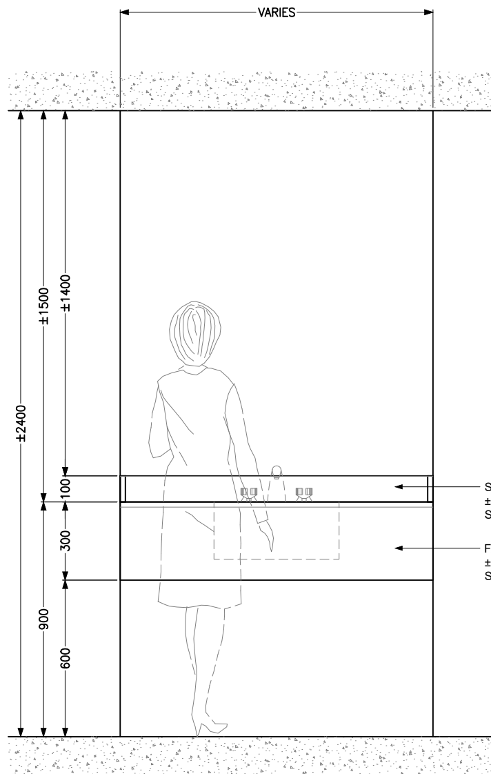
ELEVATION - PANTRY COUNTERTOP SCALE 1:20
