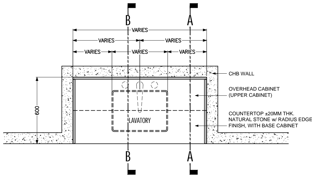
PLAN VIEW - PANTRY COUNTERTOP SCALE 1:20
