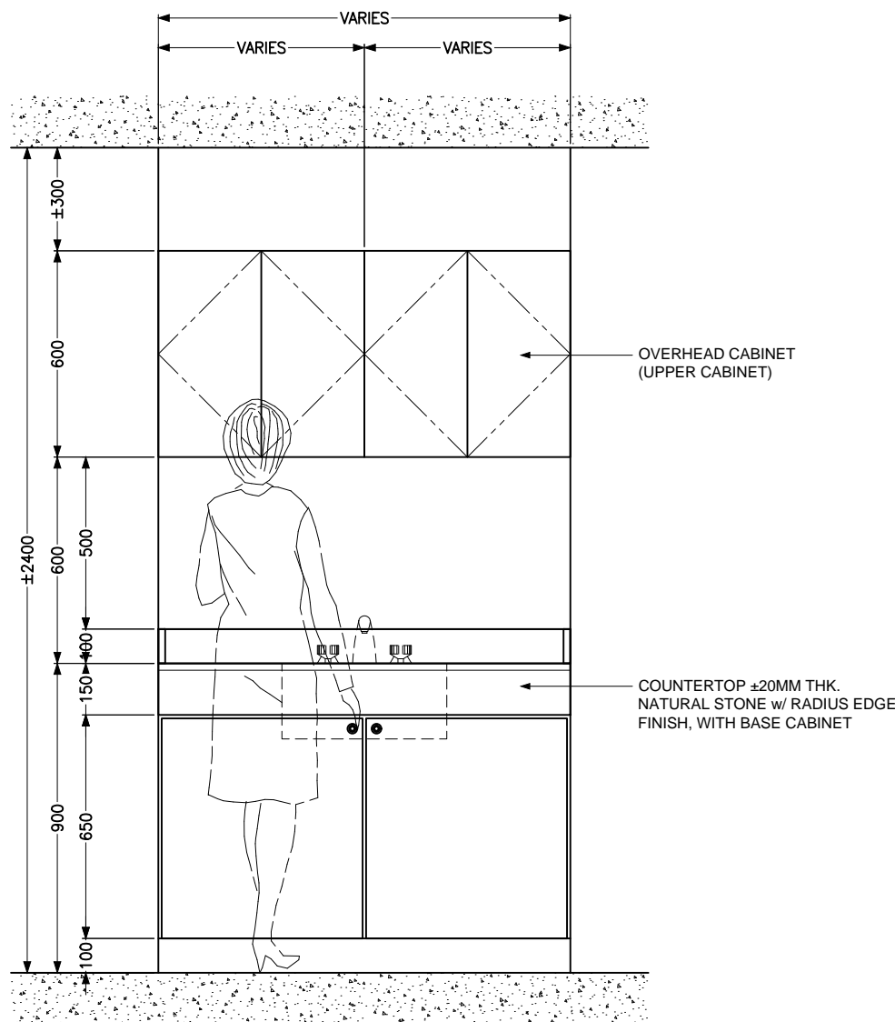
ELEVATION - PANTRY COUNTERTOP SCALE 1:20
