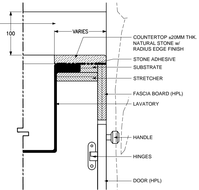
SPOT DETAIL 2 SCALE 1:5
