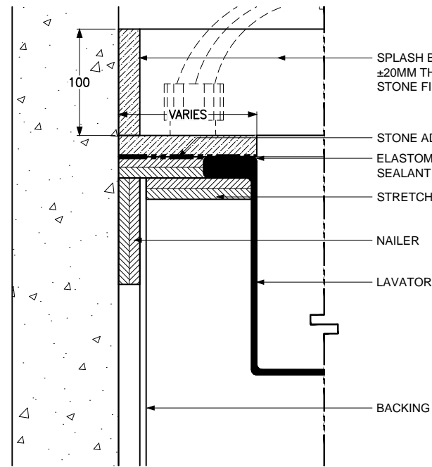
SPOT DETAIL 1 SCALE 1:5
