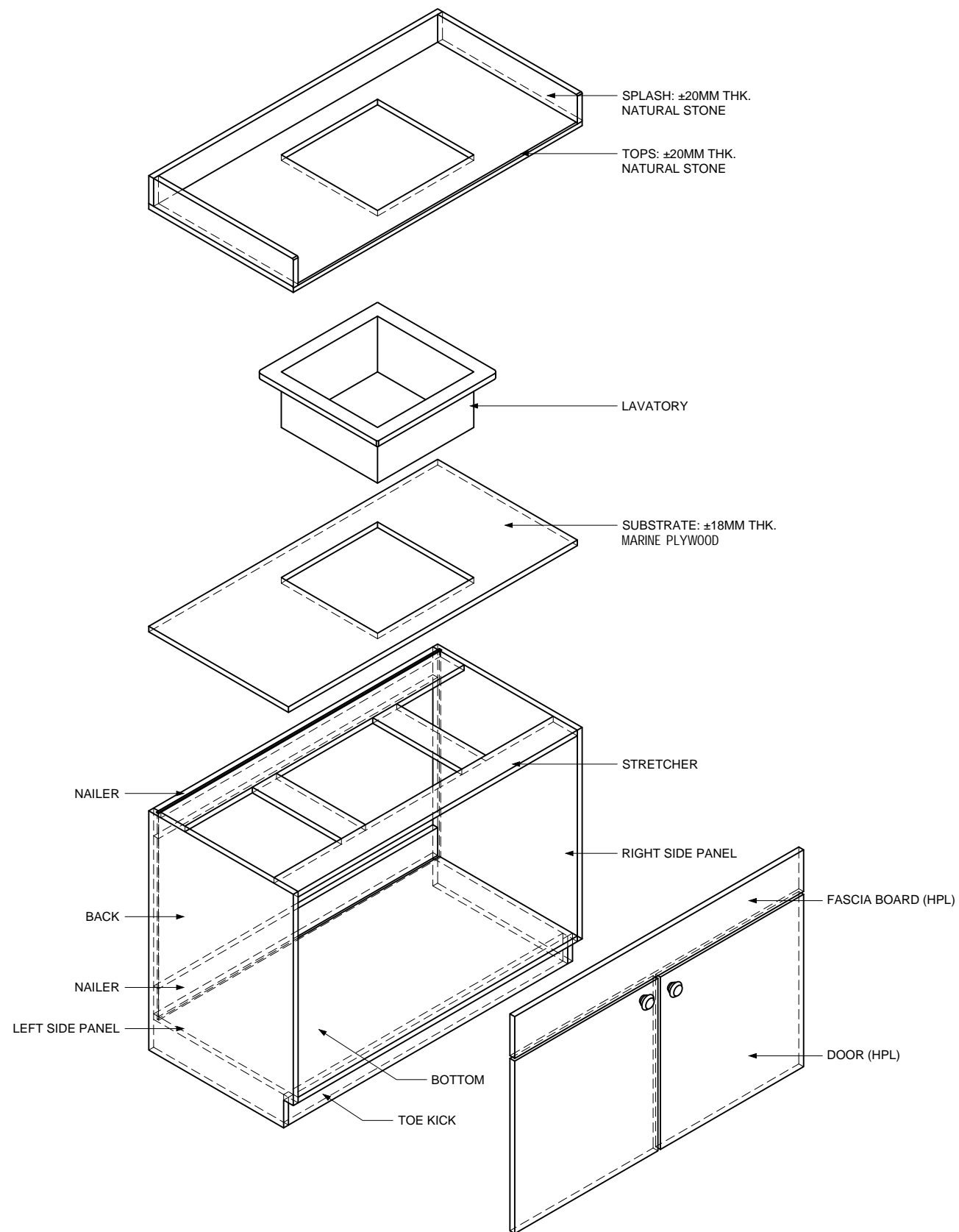
COUNTERTOP ASSEMBLY DRAWING SCALE 1:20
