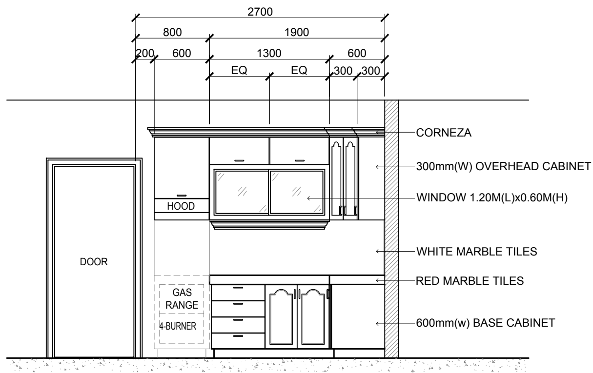
INTERIOR ELEVATION A
