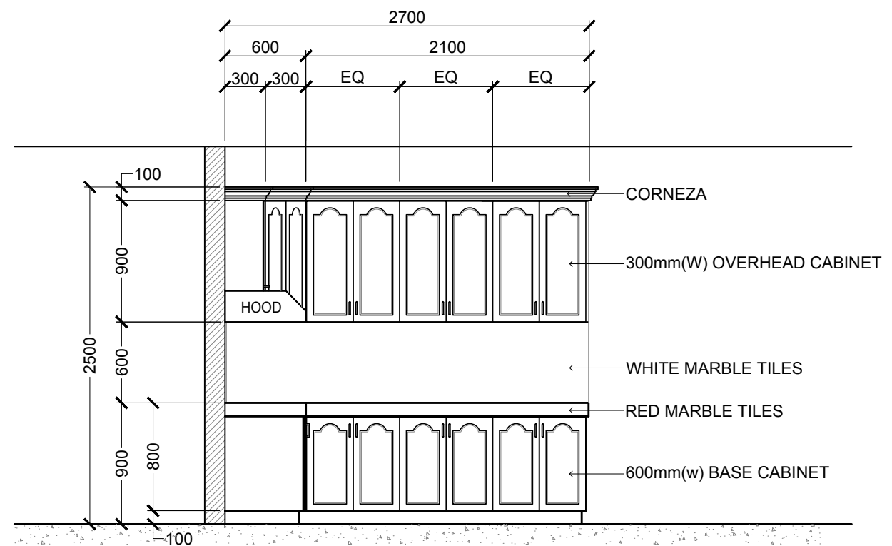
INTERIOR ELEVATION B
